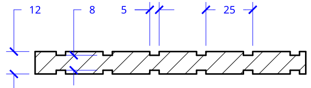
A - A BATTEN PANEL
