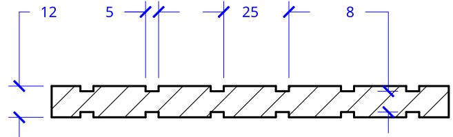
A - A BATTEN PANEL
