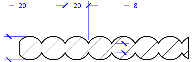
A - A ARC PANEL
