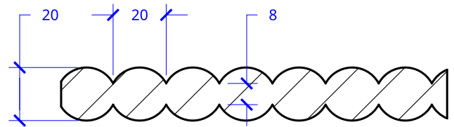
A - A ARC PANEL
